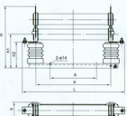
RN5-3/150-200, RN5-6/100-200 RN5-10/75-100型外形尺寸
