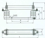
RN5-3/30-100, RN5-6/30-75 RN5-10/30-50型外形尺寸
