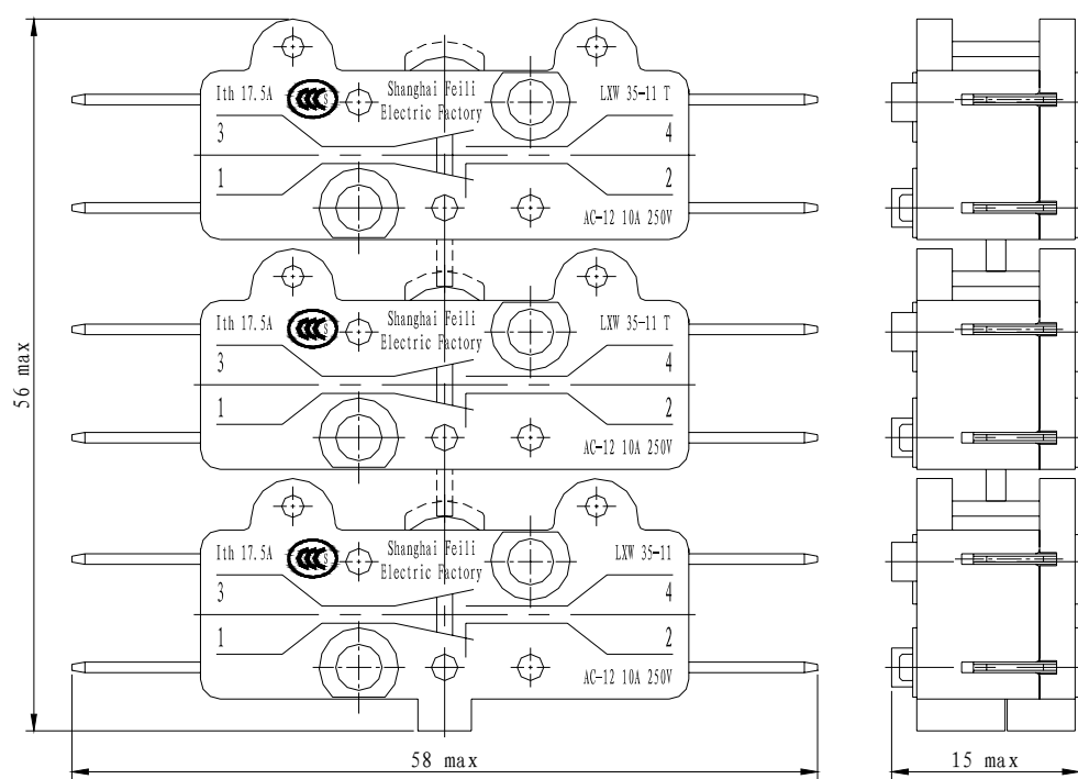
图14 三只开关组合成一组 Three switch combinations in together
